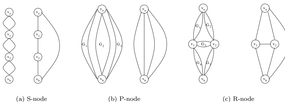
Figure 1: Pertinent graphs and skeletons of the different node types of an SPQR-tree
