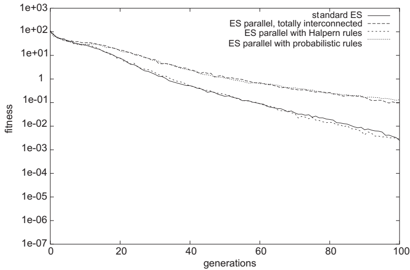
Figure 7. Comparison of the parallel ES variants.
