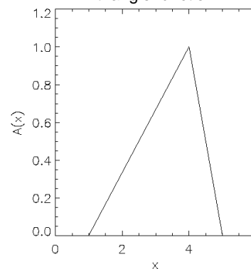
triangle function
