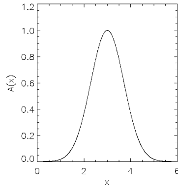
gaussoid function
