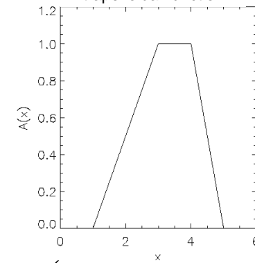
trapezoidal function
